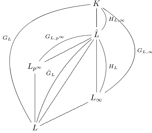
Figure 2: Galois groups of field extensions
